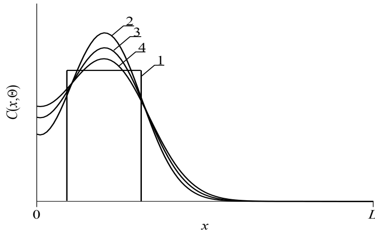
Figure 5. Spatial distributions of dopant in heterostructure after ion implantation. Curve 1 is idealized distribution of dopant. Curves 2-4 are real distributions of dopant for different values of annealing time. Increasing of number of curve corresponds to increasing of annealing time.
