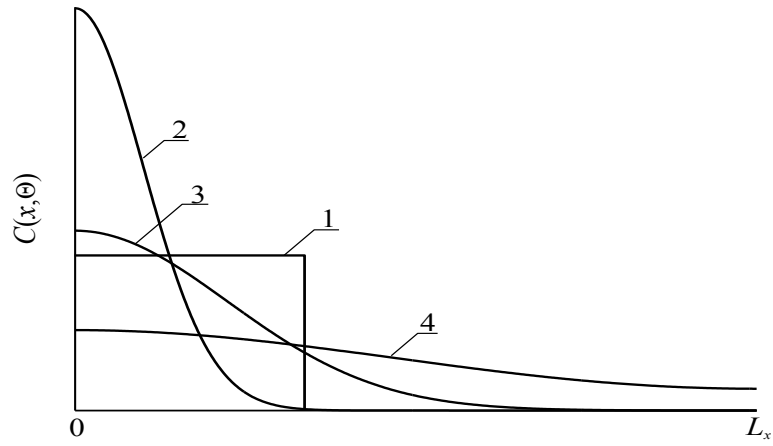
Figure 4. Spatial distributions of dopant in heterostructure after dopant infusion. Curve 1 is idealized distribution of dopant. Curves 2-4 are real distributions of dopant for different values of annealing time. Increasing of number of curve corresponds to increasing of annealing time.
