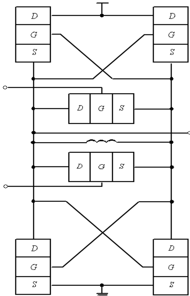
Figure 1. Structure of the considered divider.
