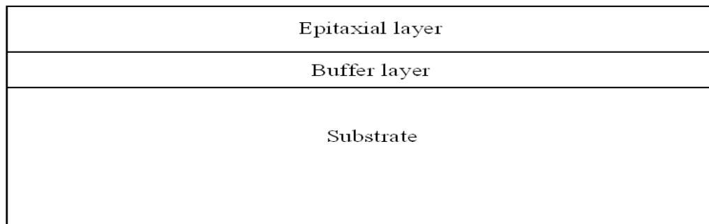
Figure 2. Heterostructure with a substrate, epitaxial layers and buffer layer (view from side).
